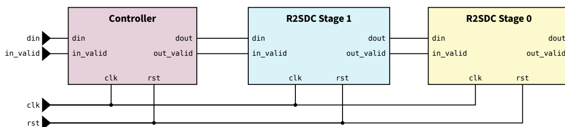
Figure 3.11: Schematic of R2SDC implementation
