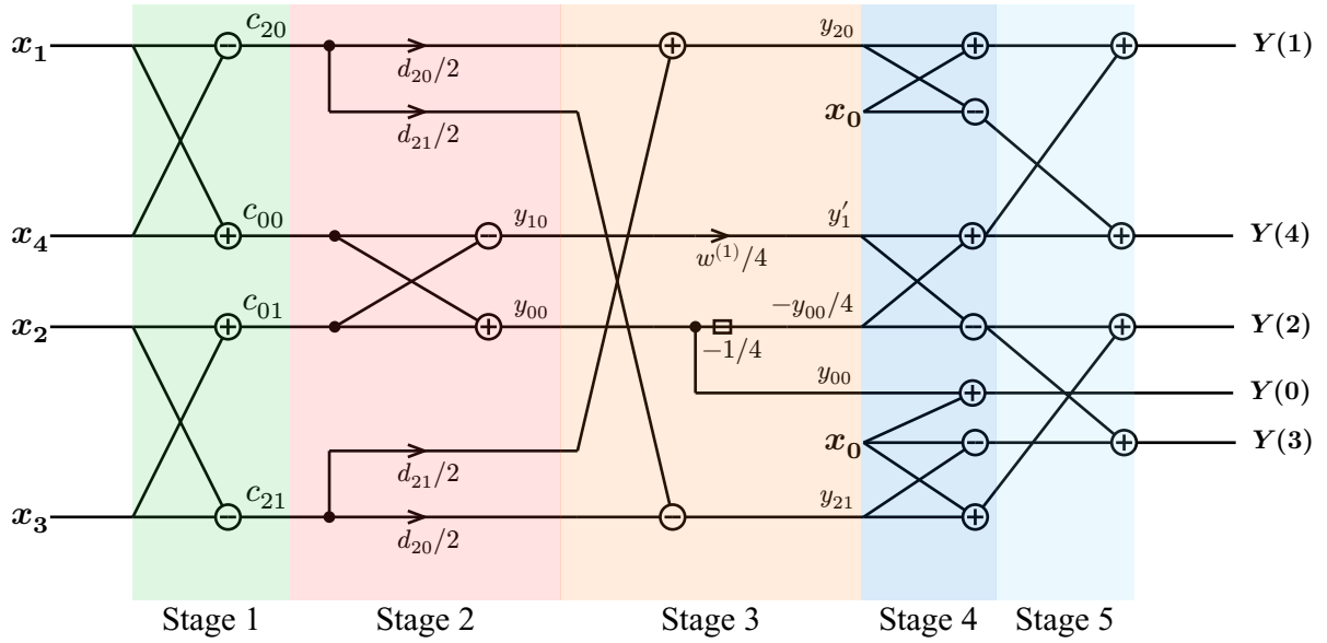
Figure 3.15: Signal flow of modified Winograd algorithm for 5 point DFT.
